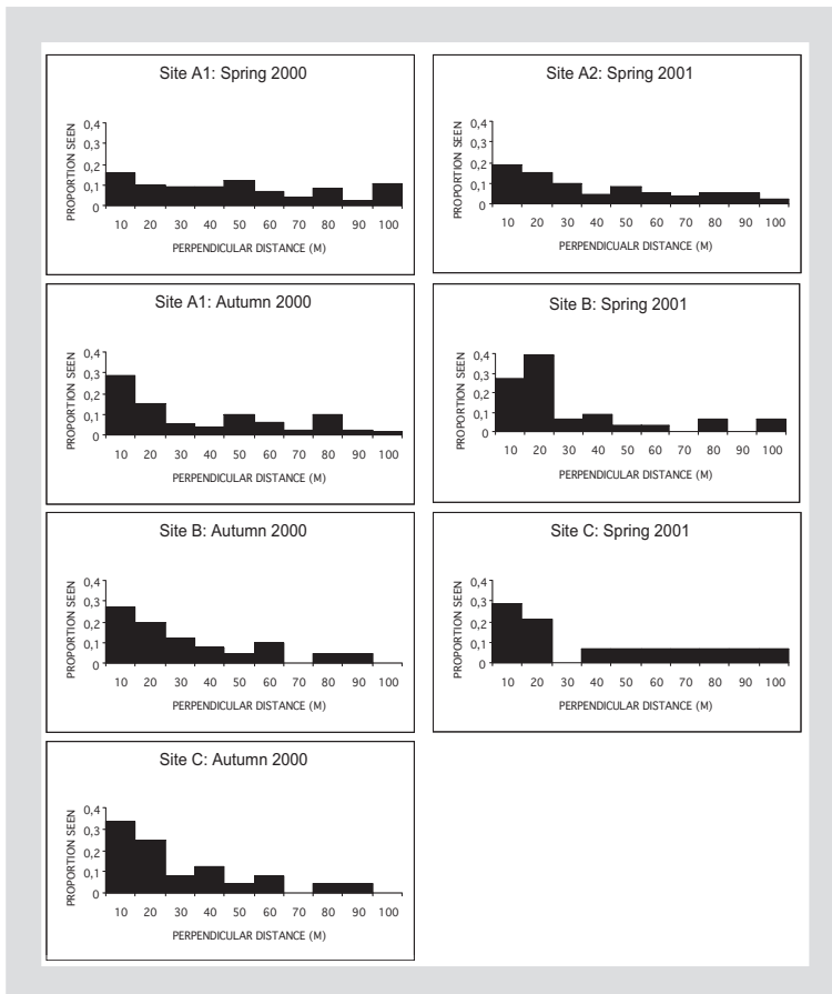
Figure 1. Histograms of perpendicular sighting distances for mountain hares on transects in the Central Highlands, Scotland.
